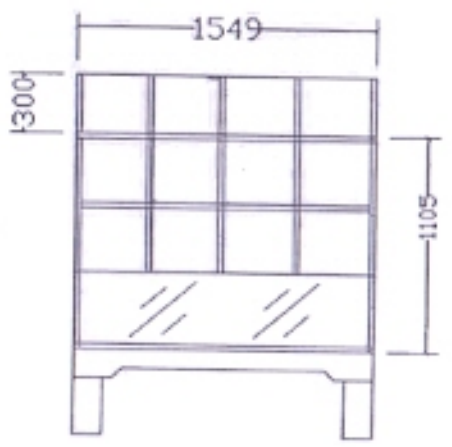
BACK ELEVATION
